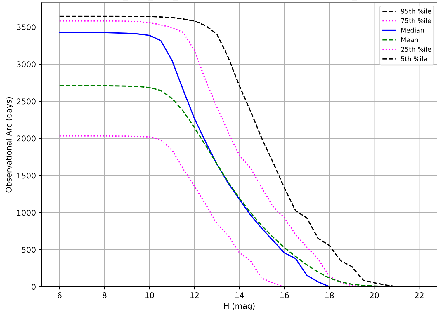
all_long_v3.4_10yrs: Observational Arc Length OCC_r5
