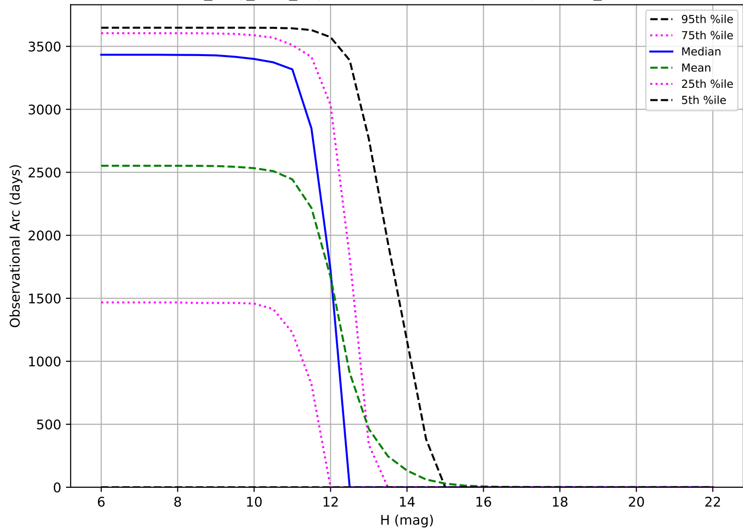
all_long_v3.4_10yrs: Observational Arc Length OCC_r20
