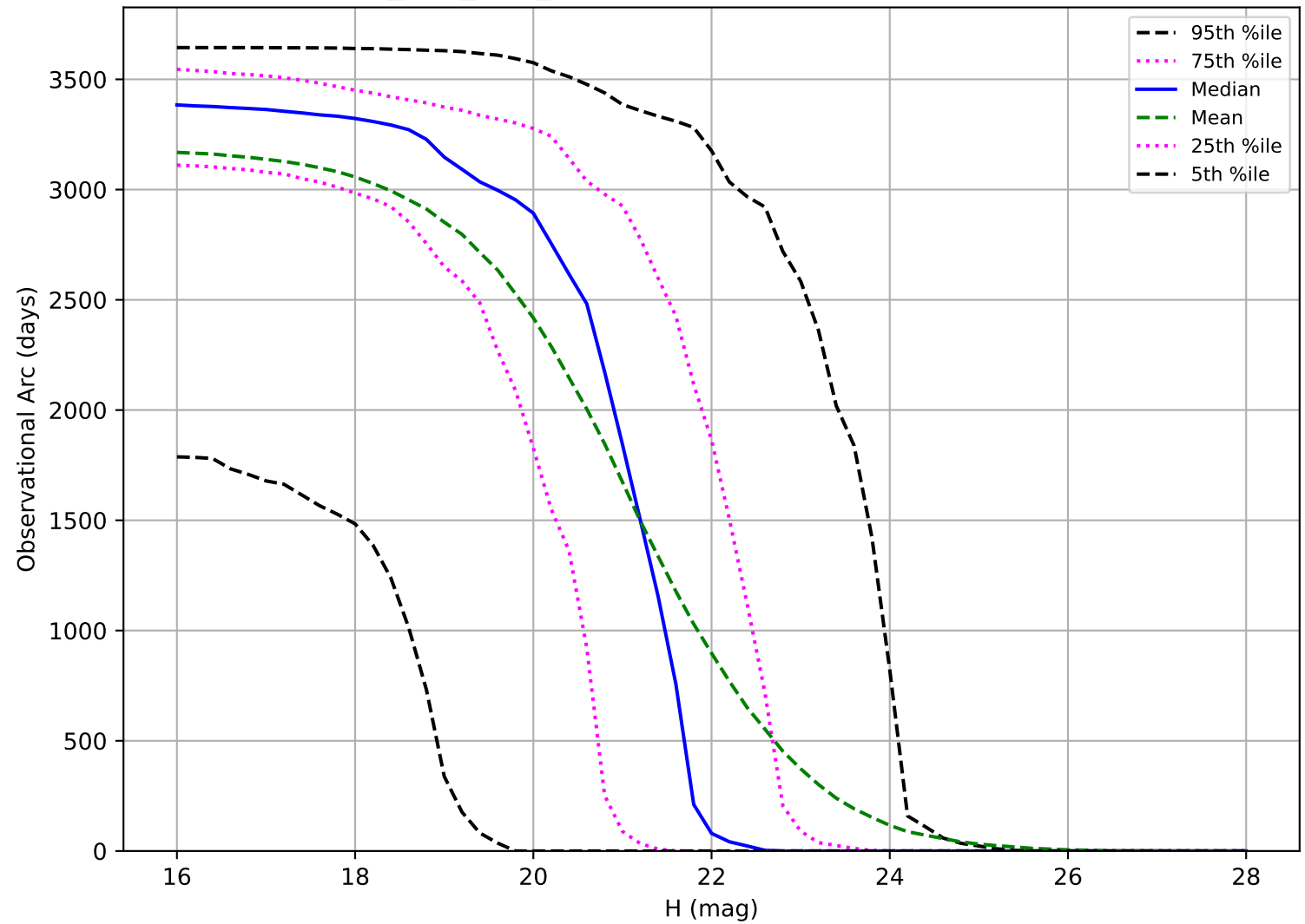
all_long_v3.4_10yrs: Observational Arc Length NEO
