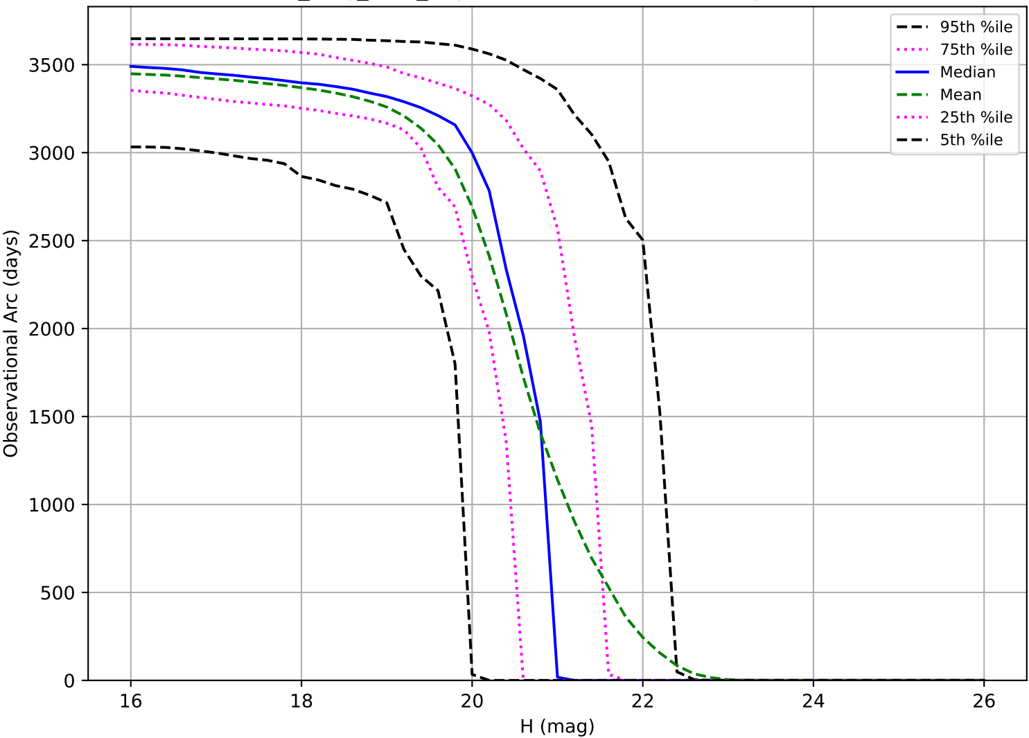
all_long_v3.4_10yrs: Observational Arc Length MBA
