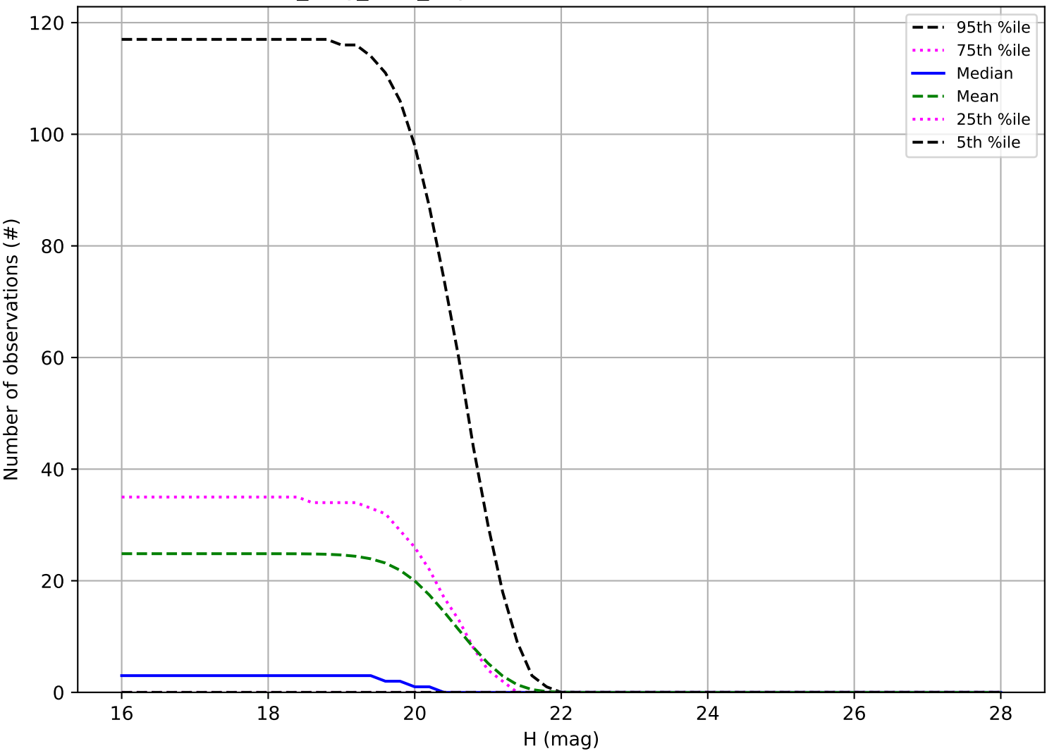
all_long_v3.4_10yrs: Number of observations Vatira
