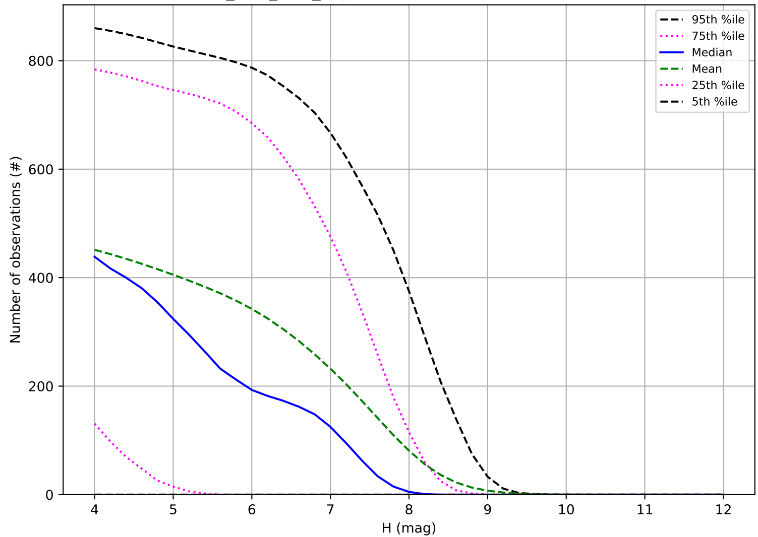
all_long_v3.4_10yrs: Number of observations TNO
