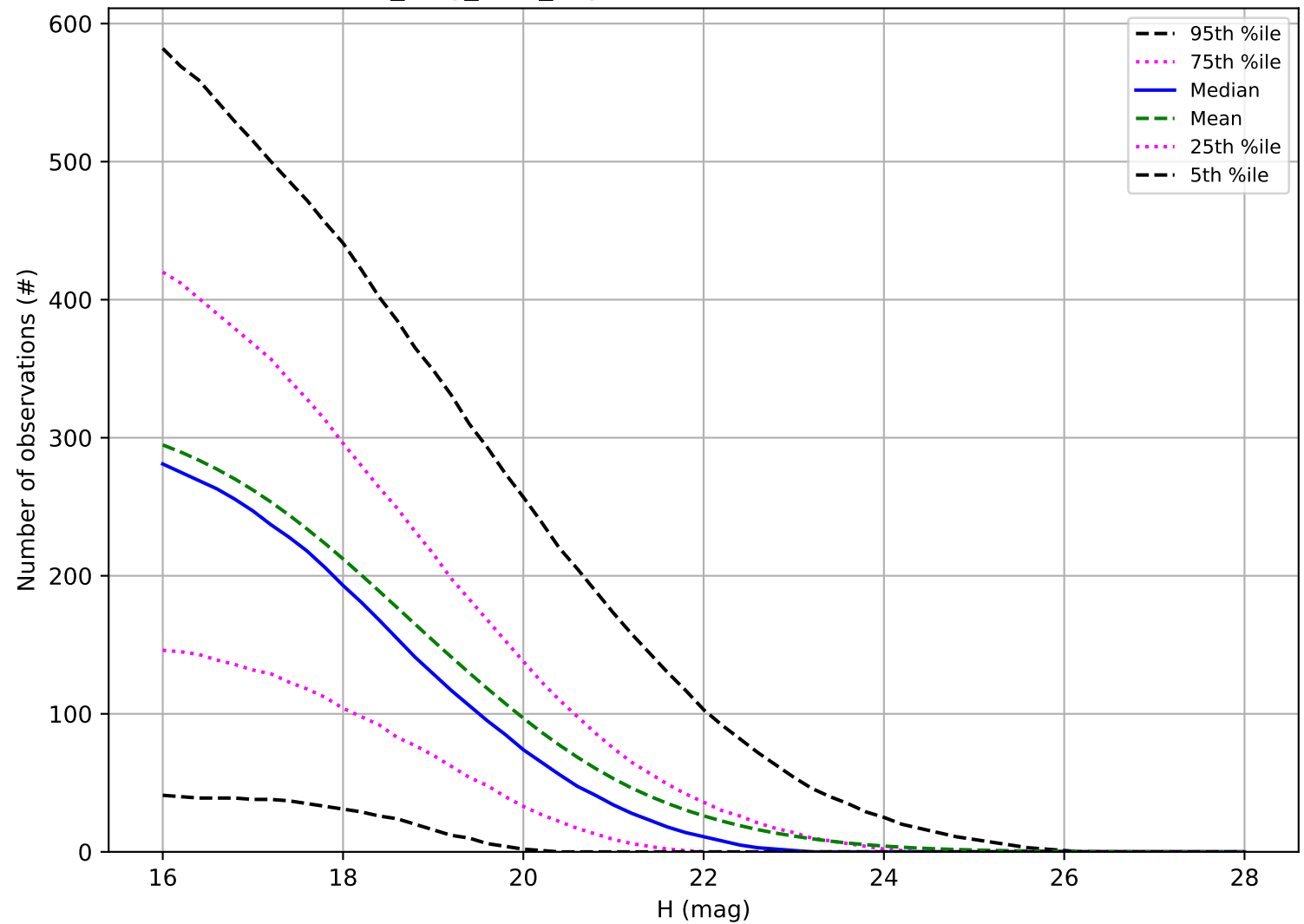
all_long_v3.4_10yrs: Number of observations PHA
