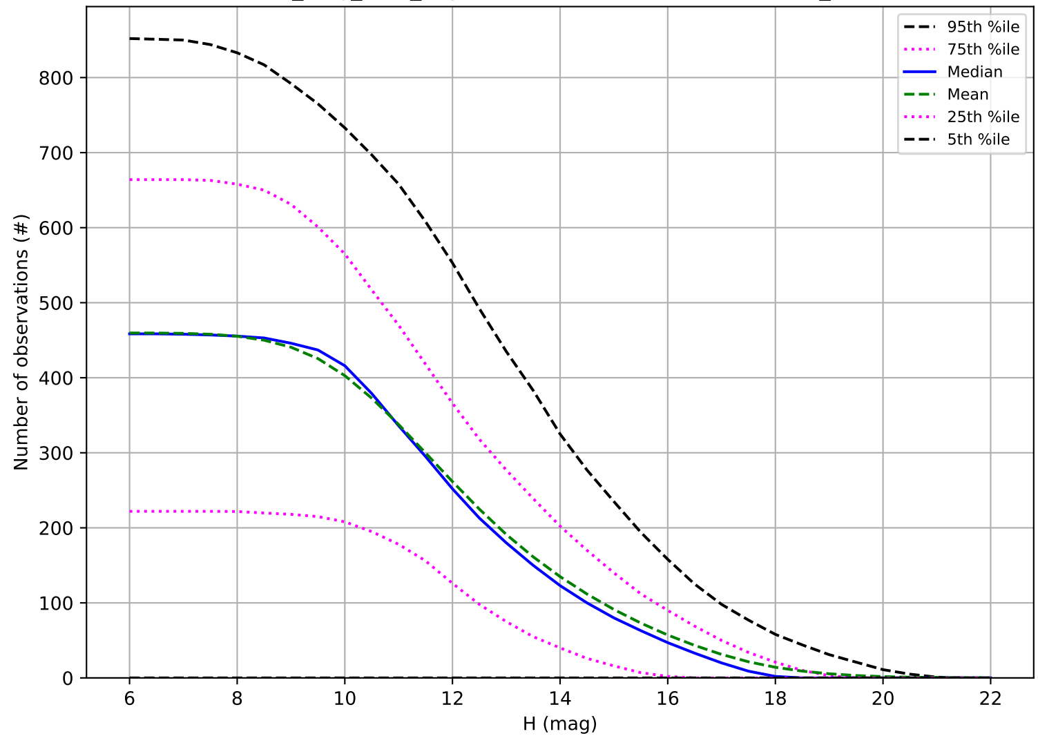
all_long_v3.4_10yrs: Number of observations OCC_r5
