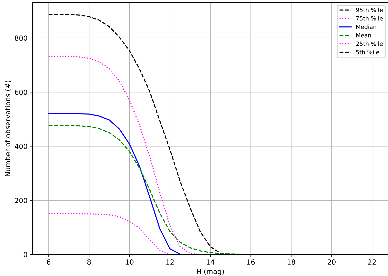
all_long_v3.4_10yrs: Number of observations OCC_r20
