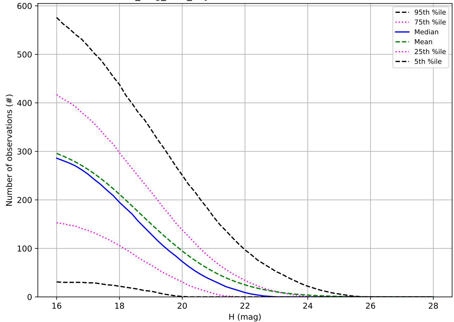
all_long_v3.4_10yrs: Number of observations NEO
