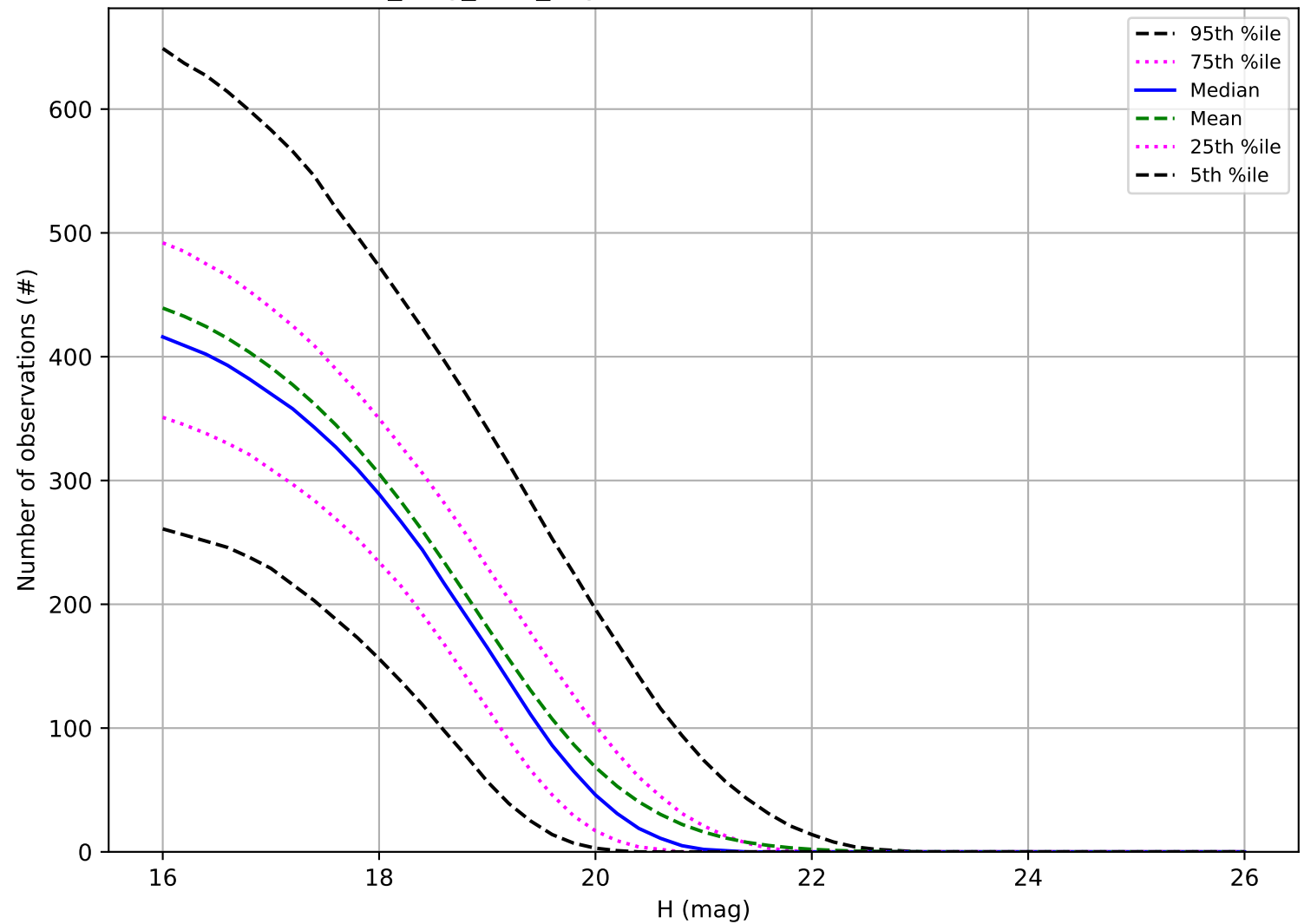
all_long_v3.4_10yrs: Number of observations MBA
