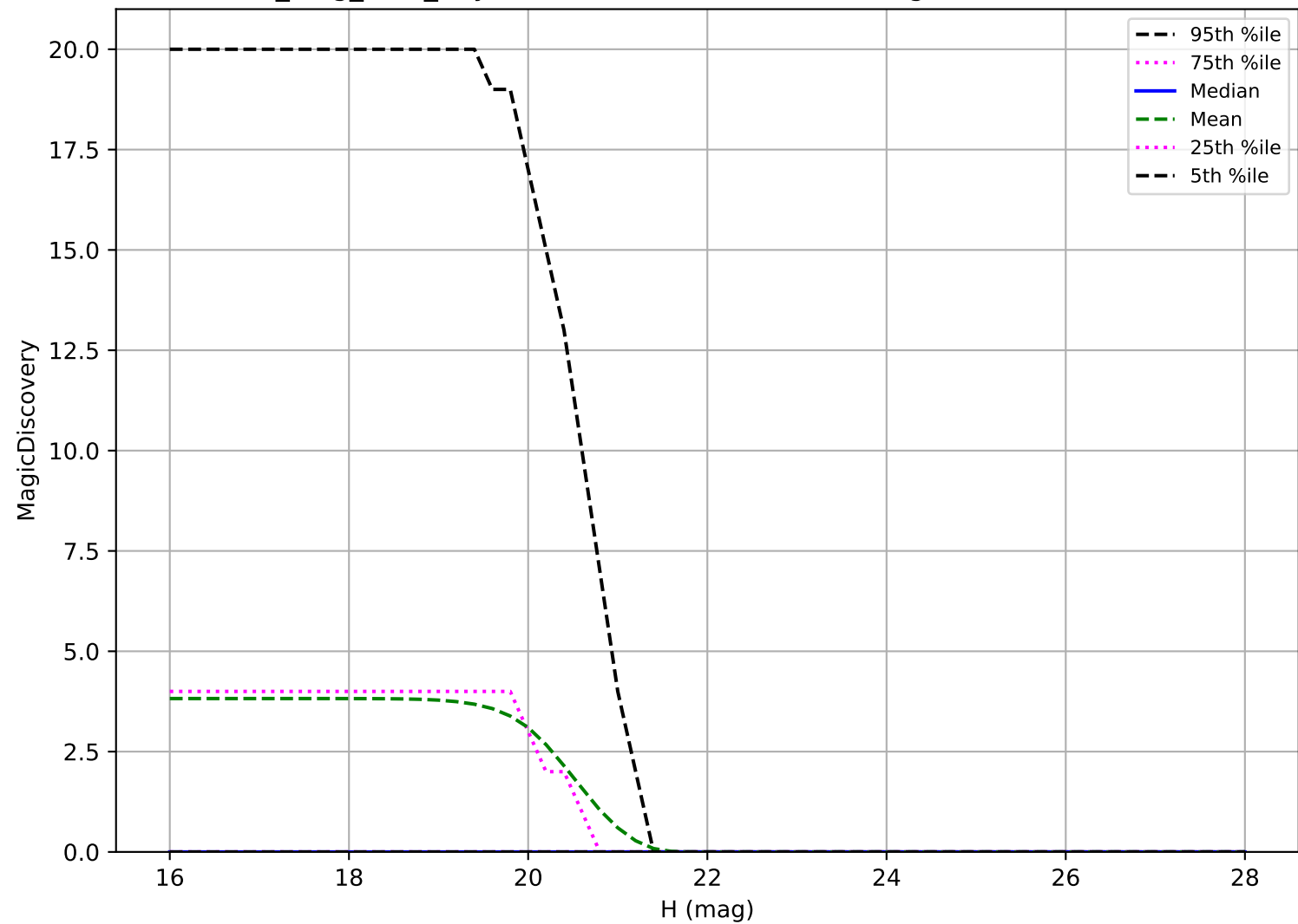
all_long_v3.4_10yrs: Vatira 6 detections in 60 nights detection loss
