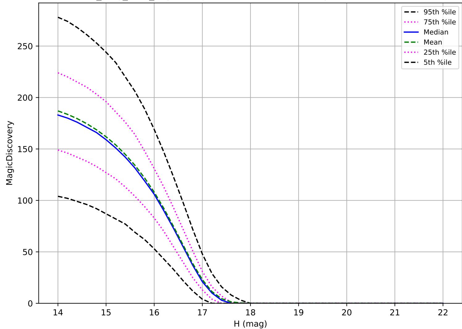
all_long_v3.4_10yrs: Trojan 6 detections in 60 nights detection loss
