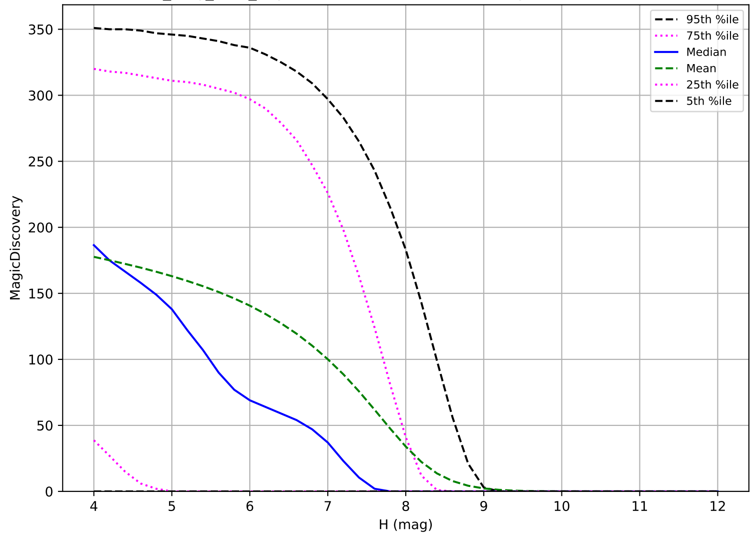
all_long_v3.4_10yrs: TNO 6 detections in 60 nights detection loss
