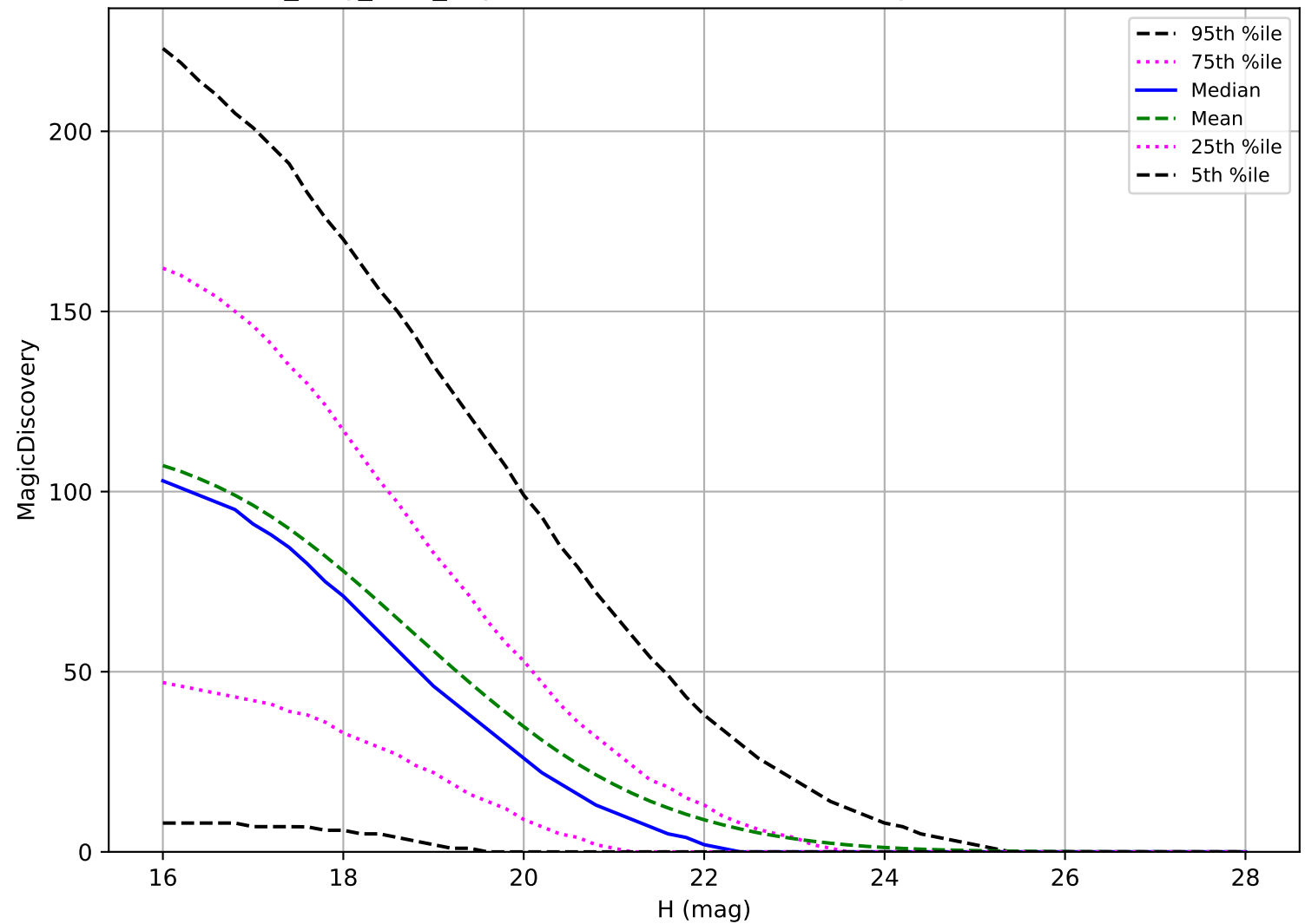
all_long_v3.4_10yrs: PHA 6 detections in 60 nights detection loss
