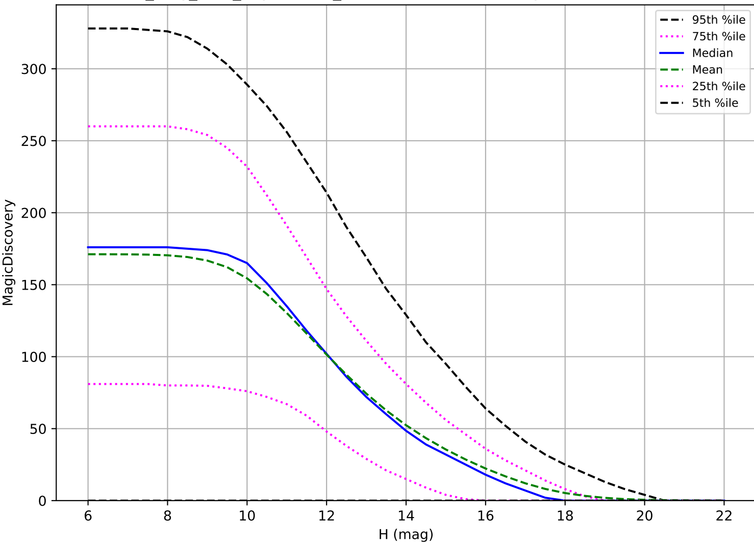
all_long_v3.4_10yrs: OCC_r5 6 detections in 60 nights detection loss
