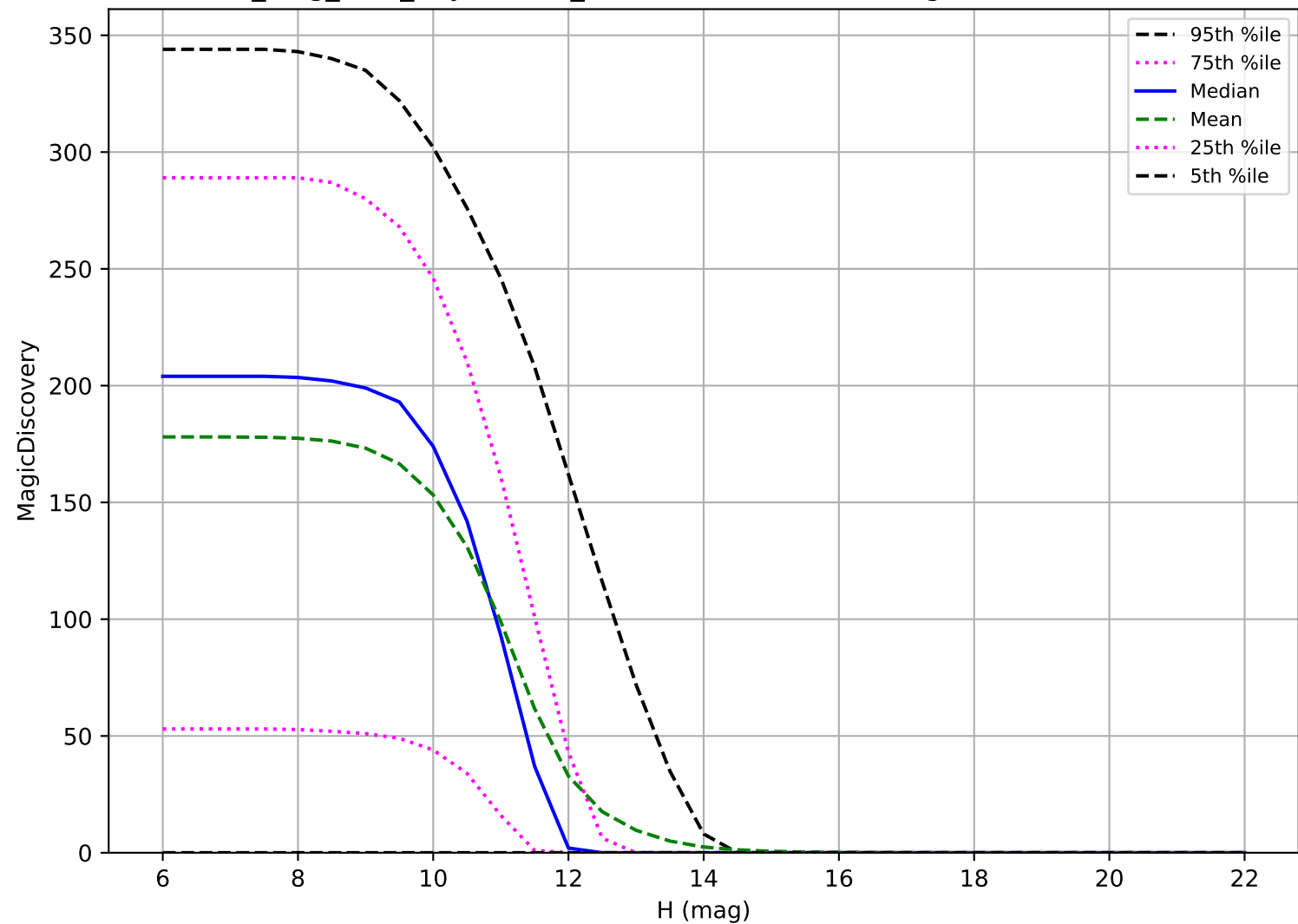
all_long_v3.4_10yrs: OCC_r20 6 detections in 60 nights detection loss
