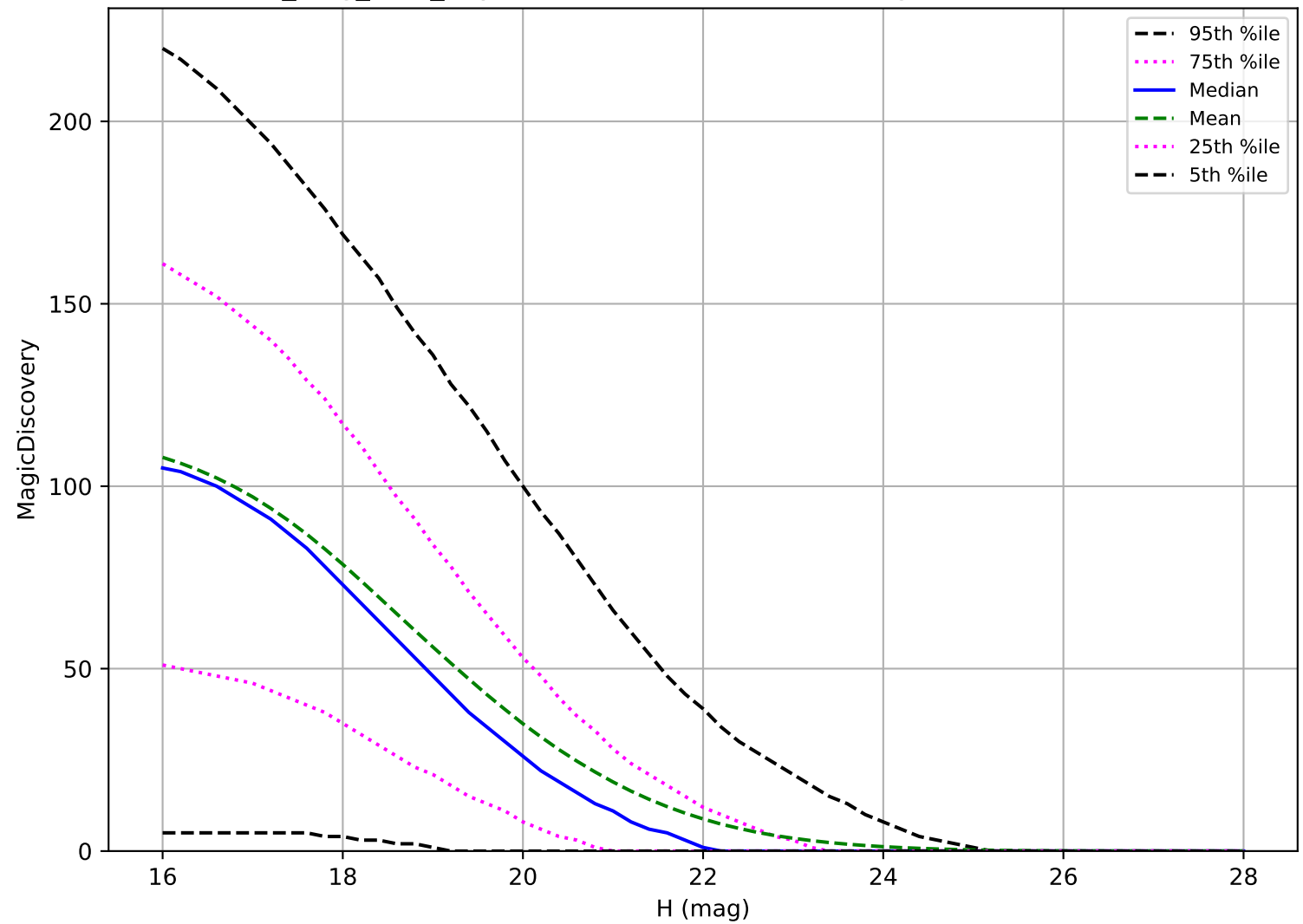
all_long_v3.4_10yrs: NEO 6 detections in 60 nights detection loss
