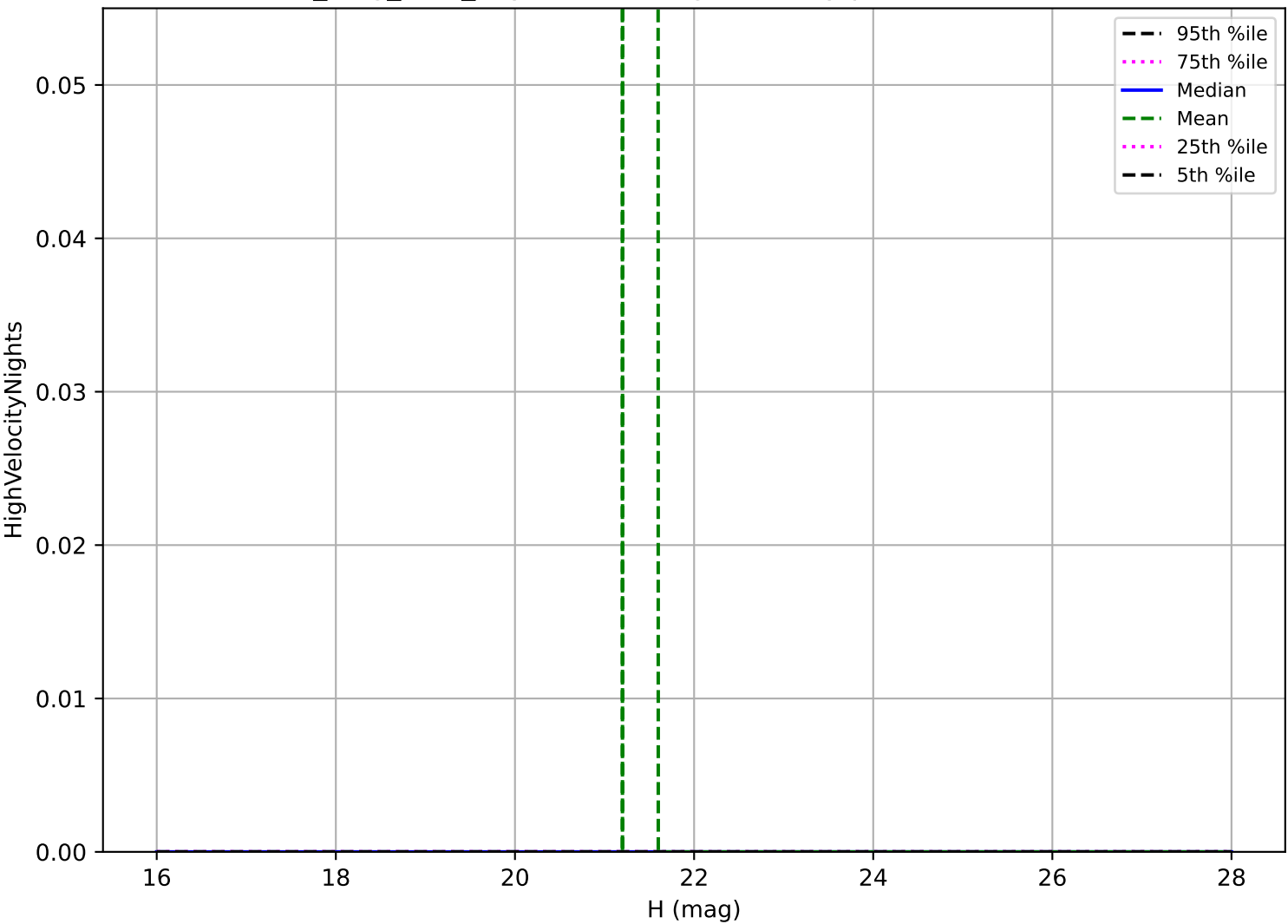
all_long_v3.4_10yrs: Vatira High velocity pair detection loss
