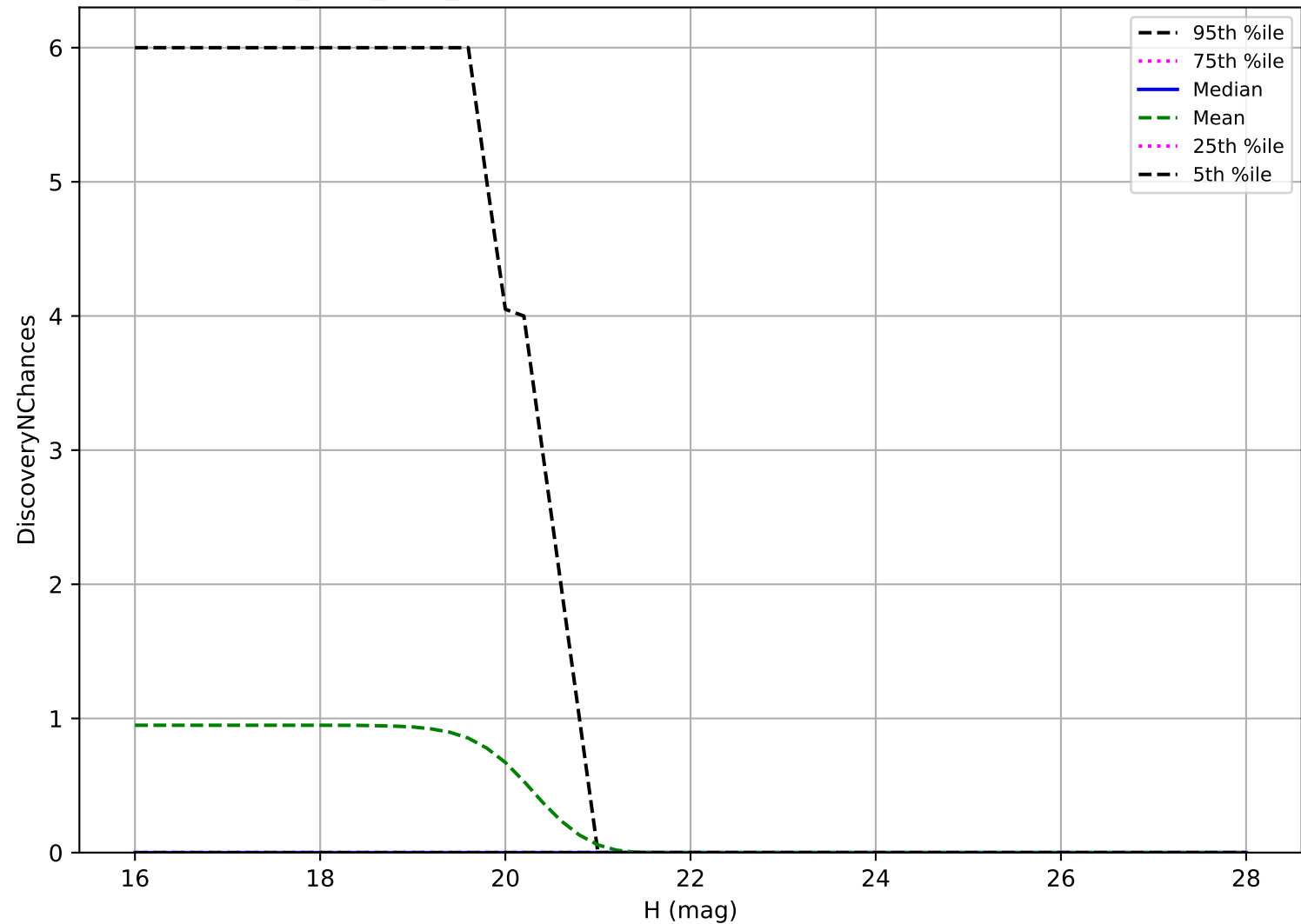
all_long_v3.4_10yrs: Vatira 3 pairs in 15 nights detection loss
