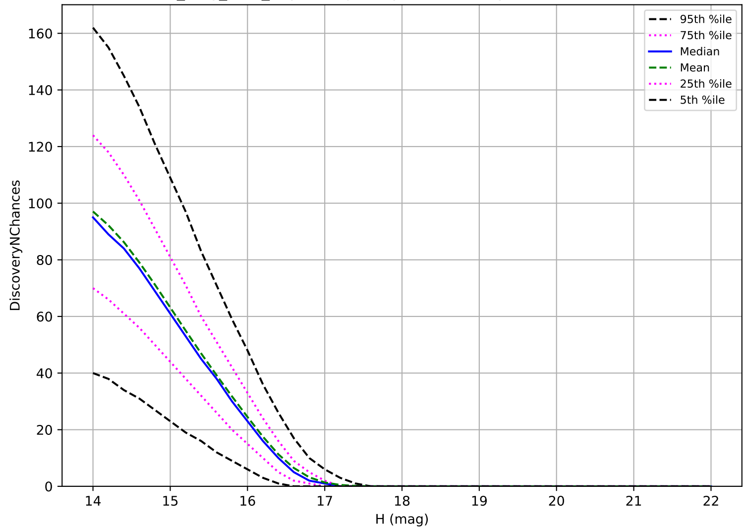
all_long_v3.4_10yrs: Trojan 3 pairs in 15 nights detection loss
