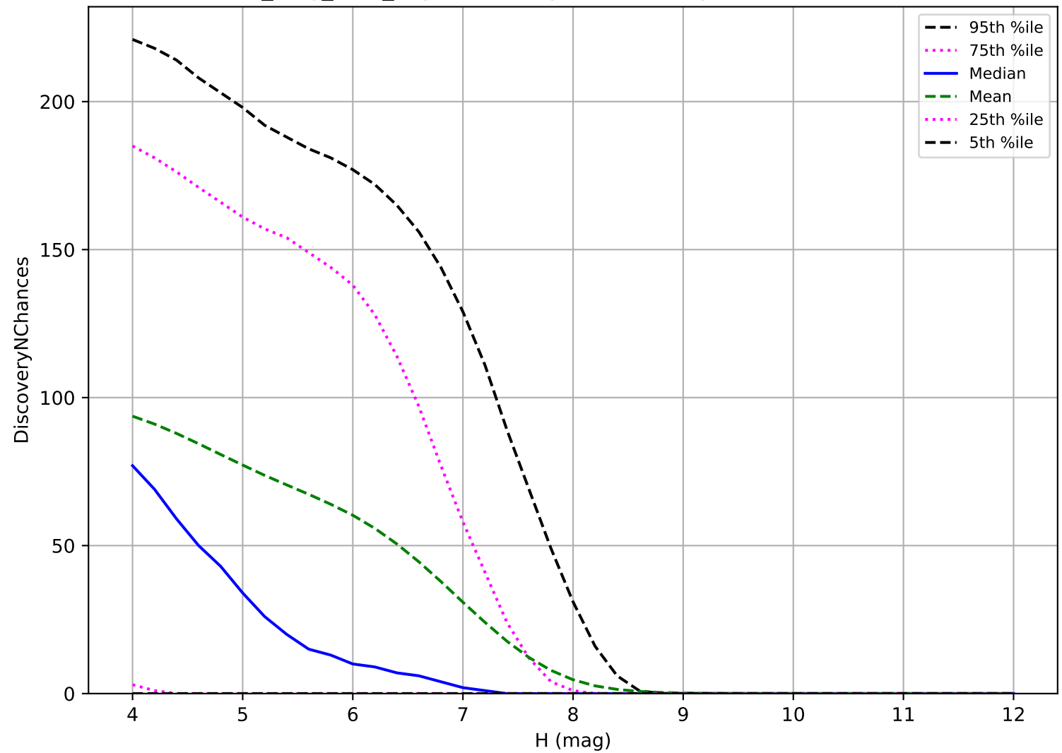
all_long_v3.4_10yrs: TNO 3 pairs in 15 nights detection loss
