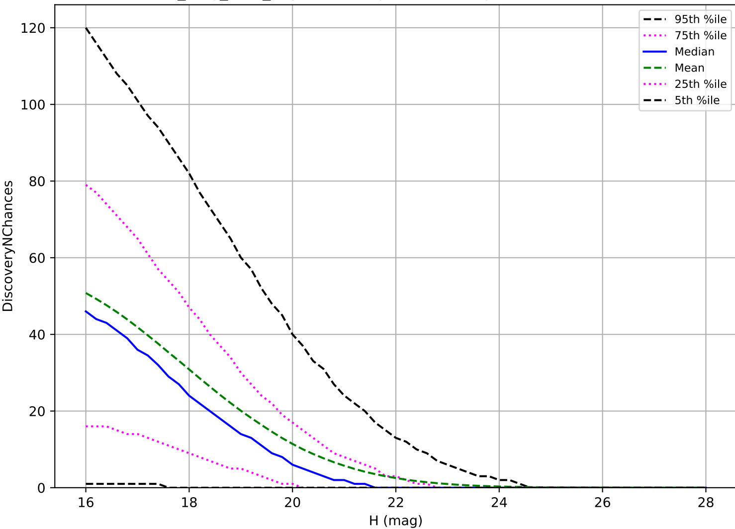
all_long_v3.4_10yrs: PHA 3 pairs in 15 nights detection loss
