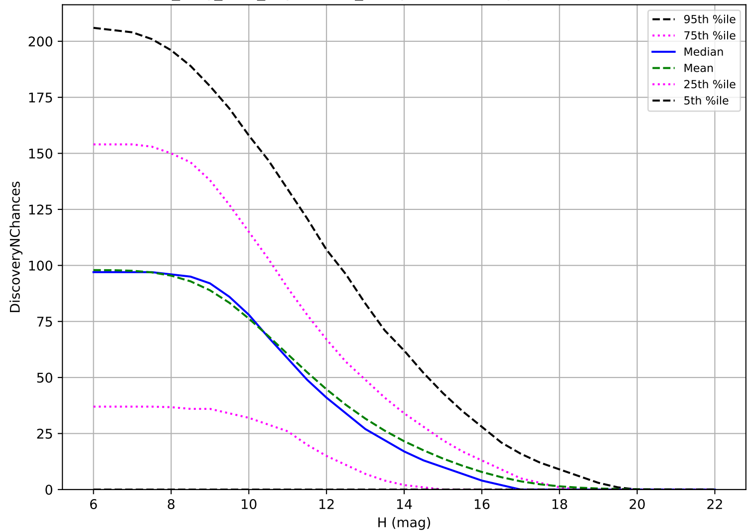
all_long_v3.4_10yrs: OCC_r5 3 pairs in 15 nights detection loss
