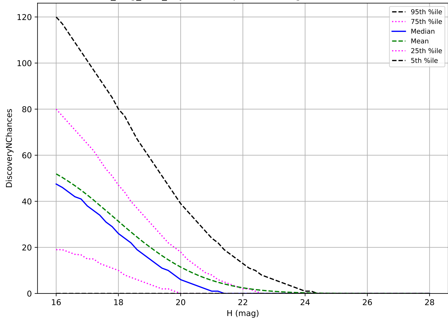
all_long_v3.4_10yrs: NEO 3 pairs in 15 nights detection loss
