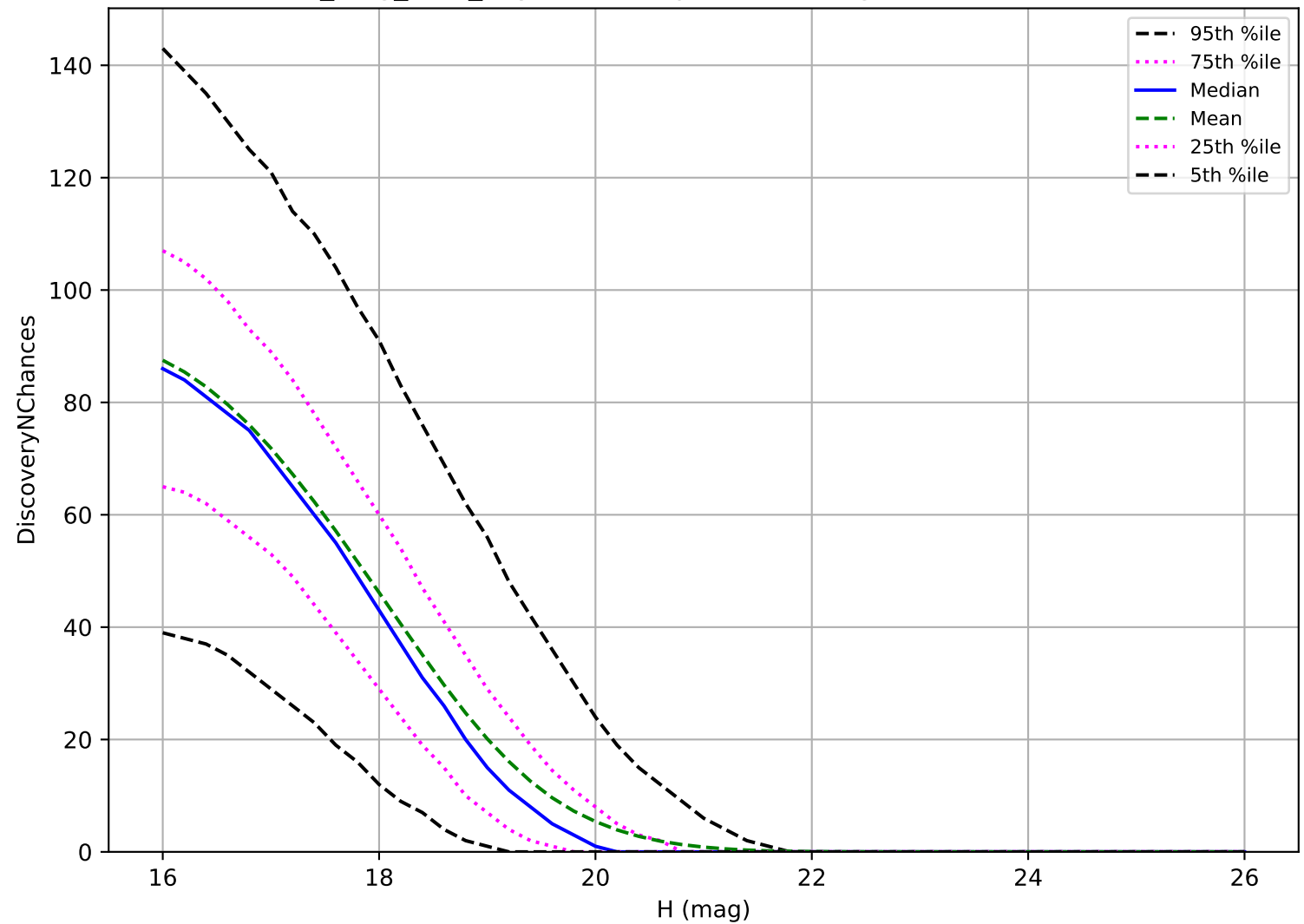
all_long_v3.4_10yrs: MBA 3 pairs in 15 nights detection loss
