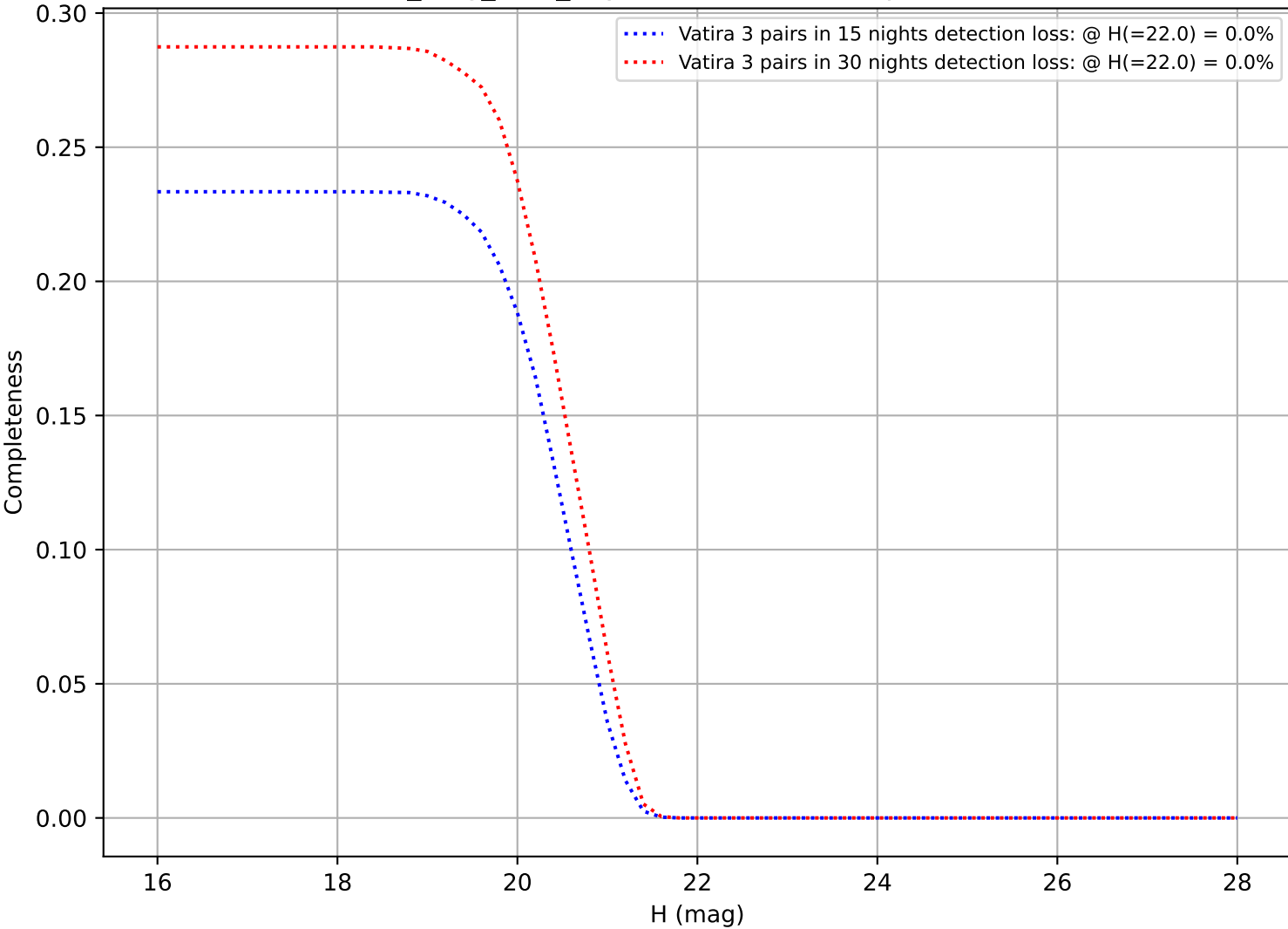
all_long_v3.4_10yrs: DifferentialCompleteness
