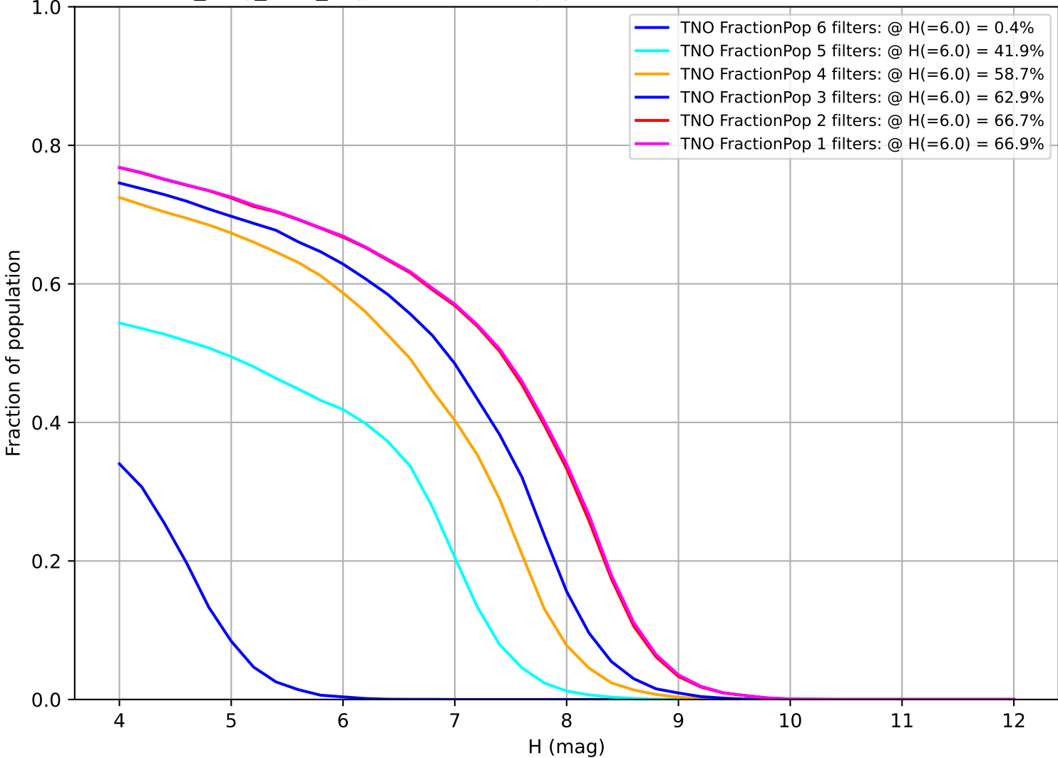
all_long_v3.4_10yrs: Fraction of population with colors in X filters TNO
