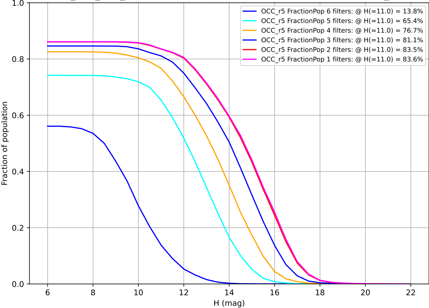
all_long_v3.4_10yrs: Fraction of population with colors in X filters OCC_r5
