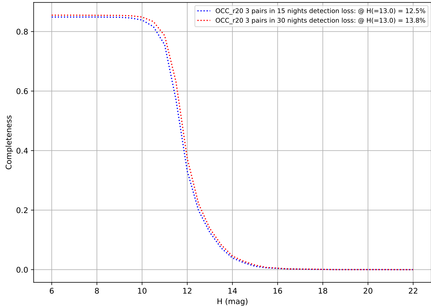
all_long_v3.4_10yrs: DifferentialCompleteness
