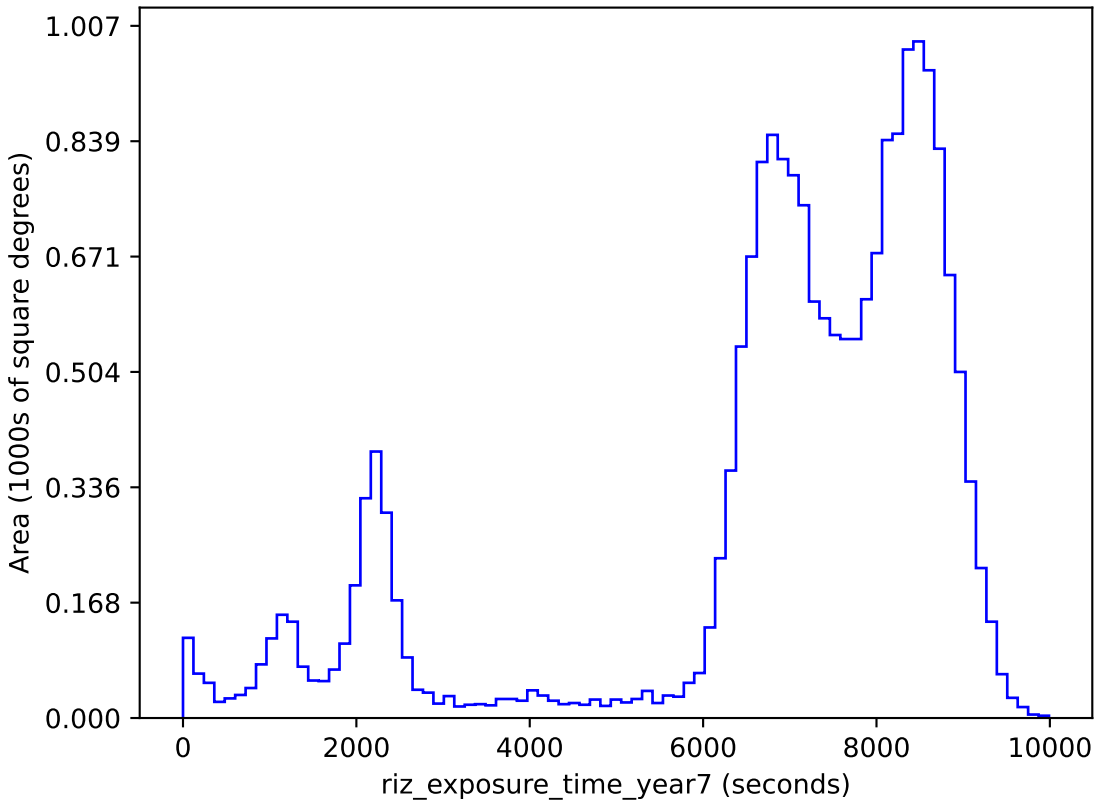
all_long_v3.4_10yrs gri band non-DD: riz_exposure_time_year7
