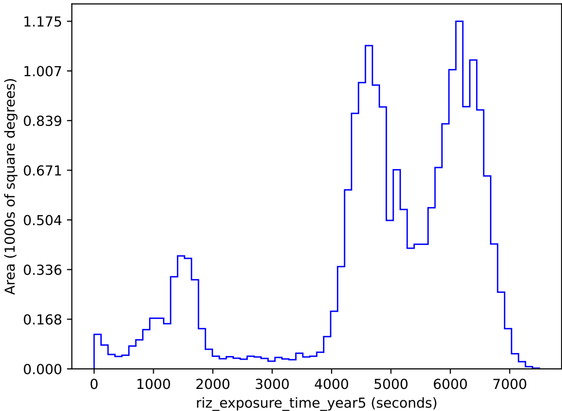
all_long_v3.4_10yrs gri band non-DD: riz_exposure_time_year5
