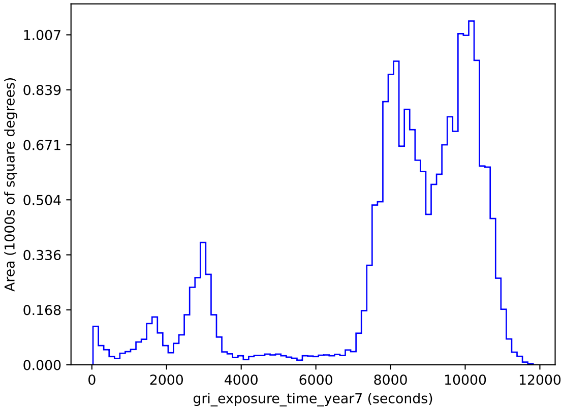
all_long_v3.4_10yrs gri band non-DD: gri_exposure_time_year7
