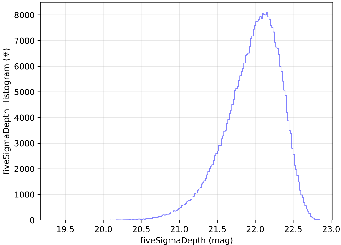
all_long_v3.4_10yrs y: fiveSigmaDepth Histogram
