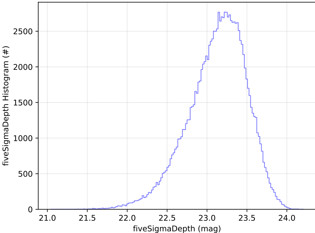
all_long_v3.4_10yrs u: fiveSigmaDepth Histogram
