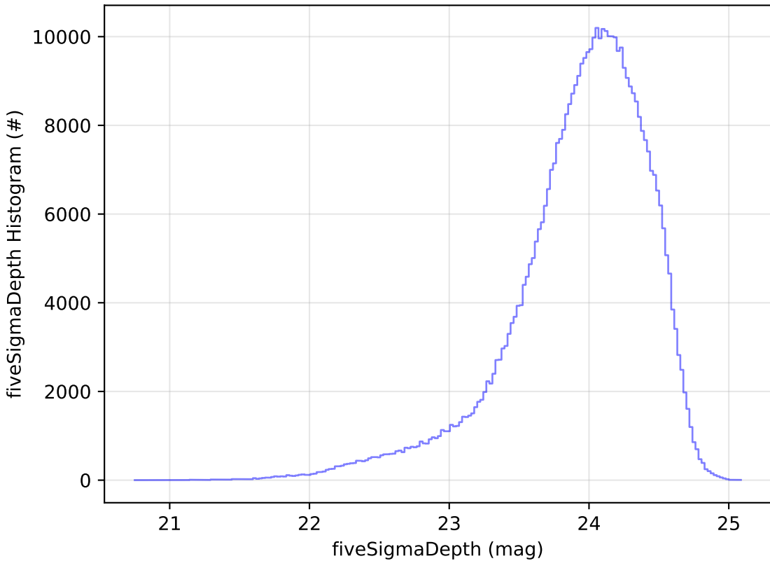
all_long_v3.4_10yrs r: fiveSigmaDepth Histogram
