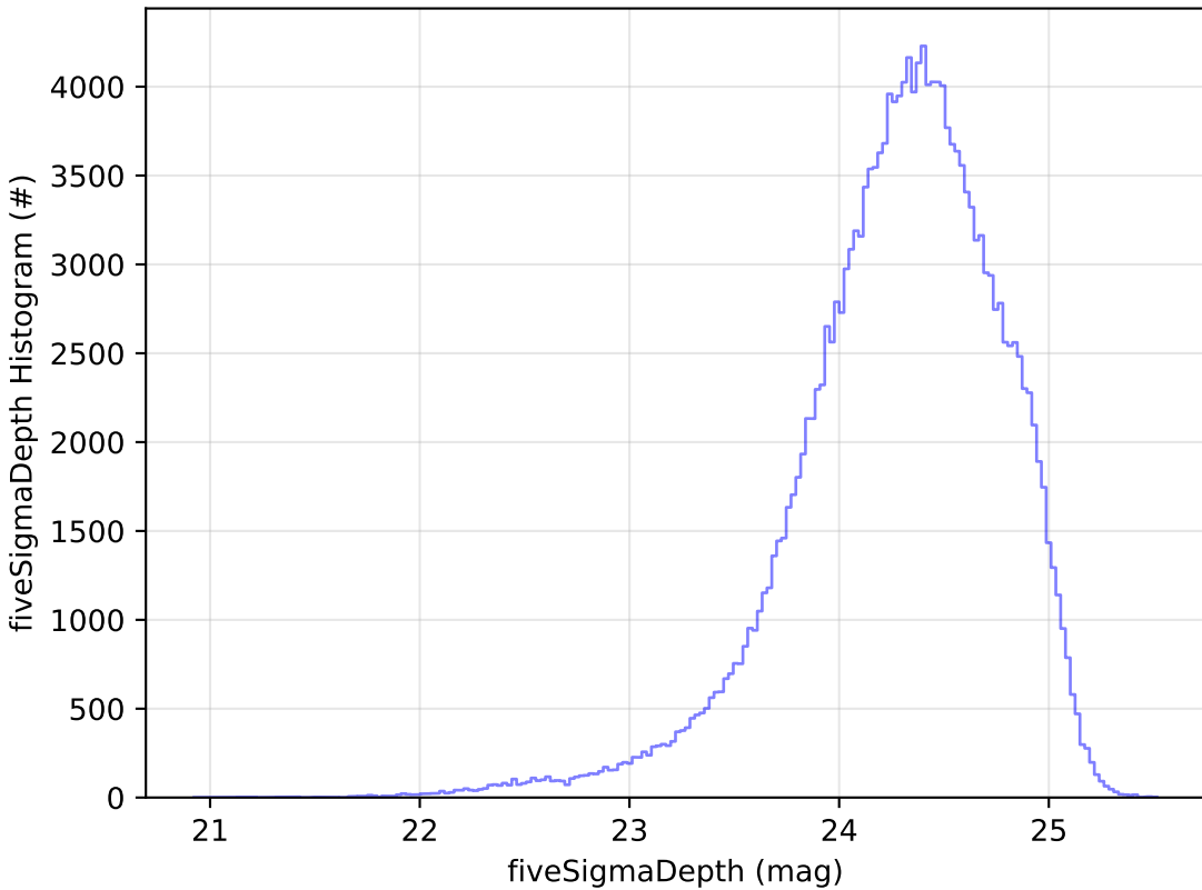
all_long_v3.4_10yrs g: fiveSigmaDepth Histogram
