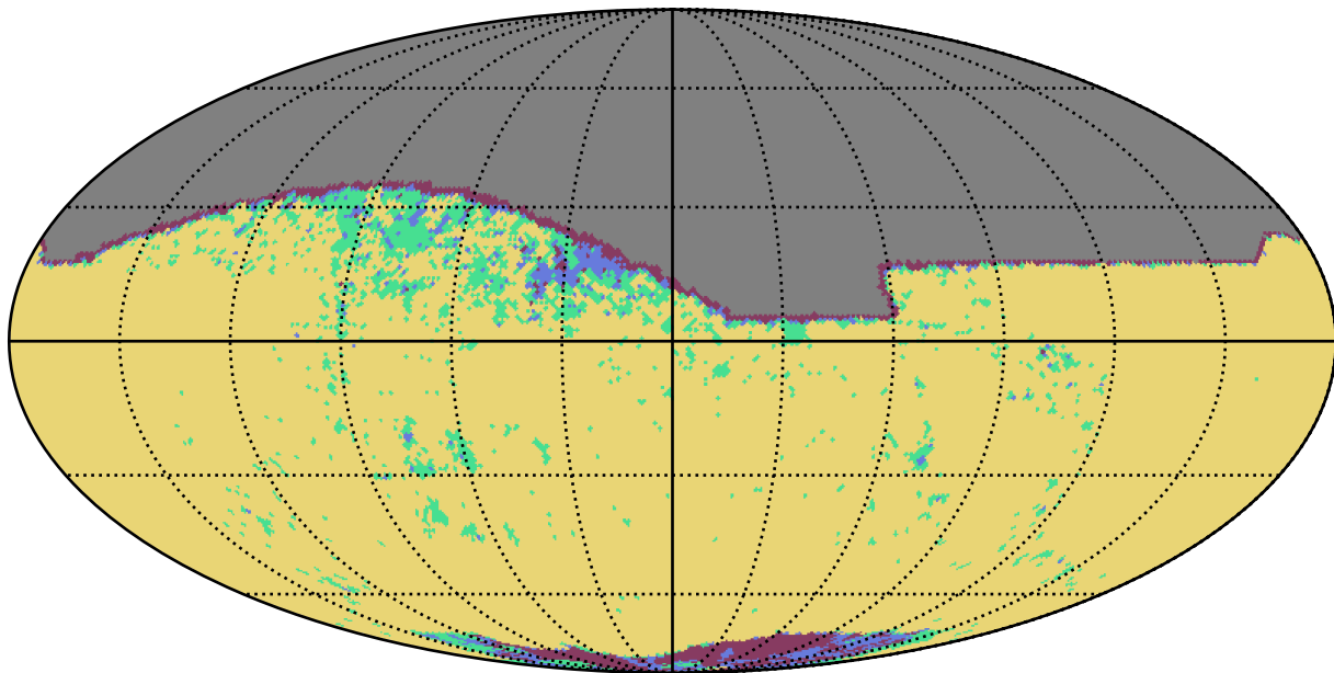
all_long_v3.4_10yrs z band: YearCoverage night
