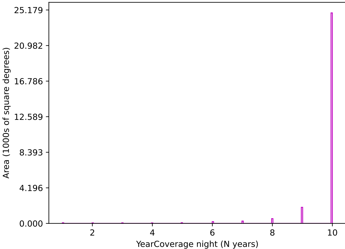
all_long_v3.4_10yrs z band: YearCoverage night
