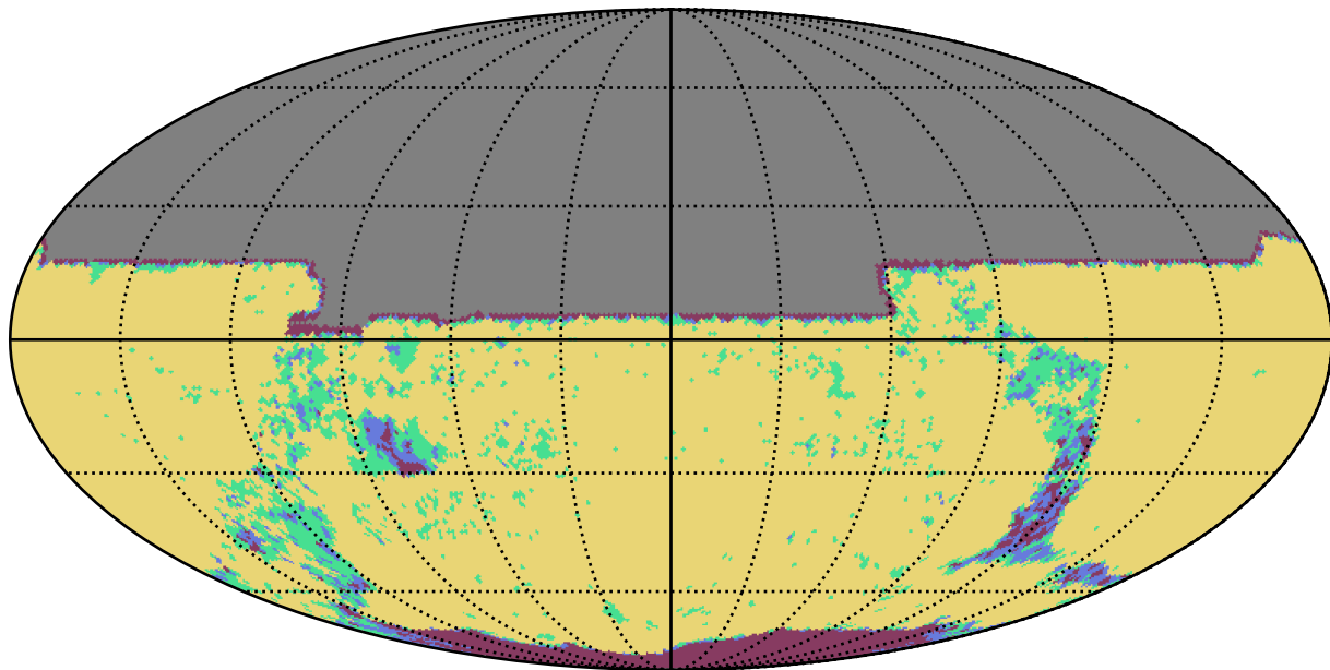
all_long_v3.4_10yrs y band: YearCoverage night
