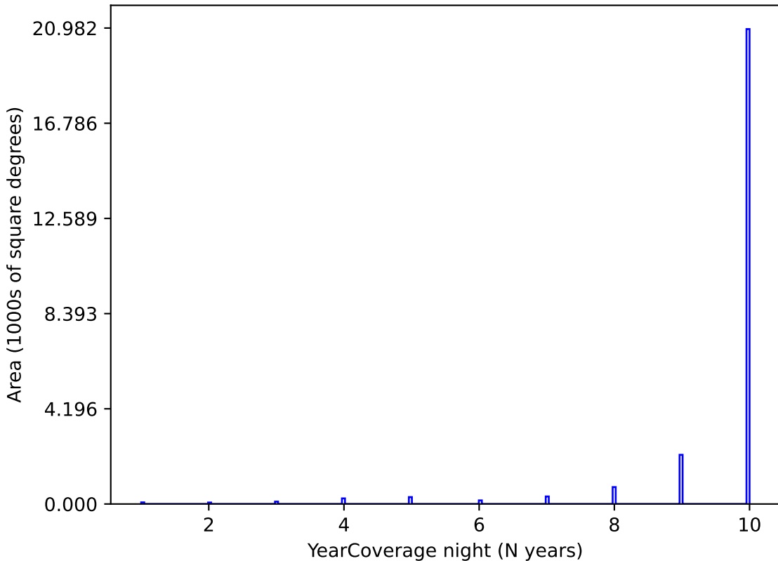
all_long_v3.4_10yrs y band: YearCoverage night
