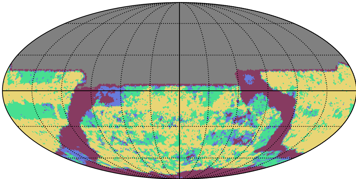
all_long_v3.4_10yrs u band: YearCoverage night
