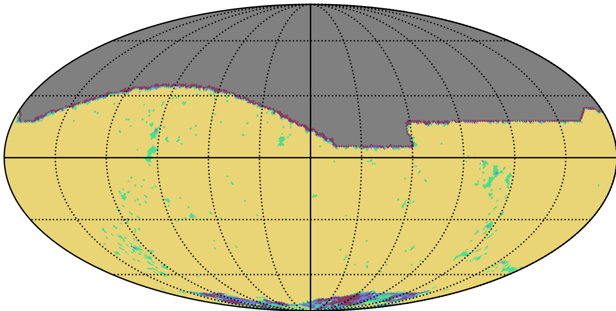
all_long_v3.4_10yrs r band: YearCoverage night
