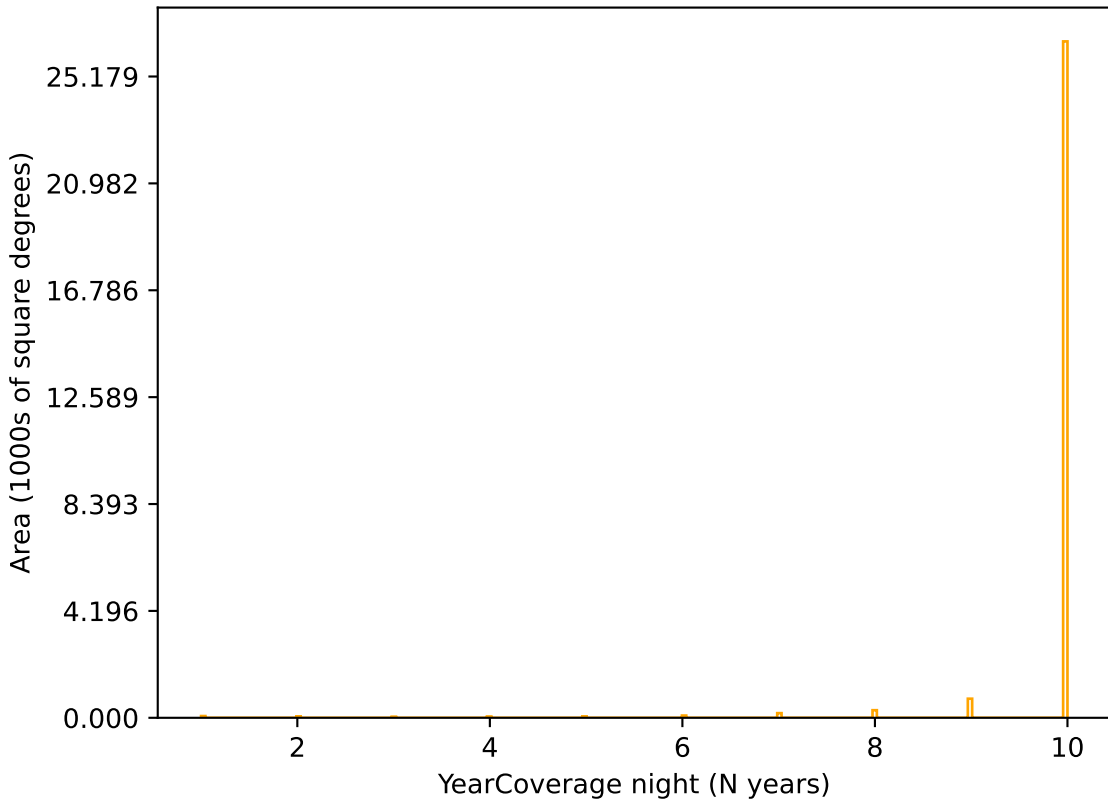
all_long_v3.4_10yrs r band: YearCoverage night
