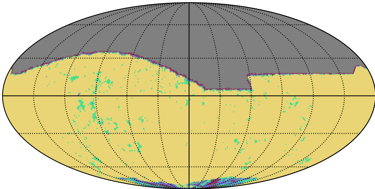
all_long_v3.4_10yrs i band: YearCoverage night
