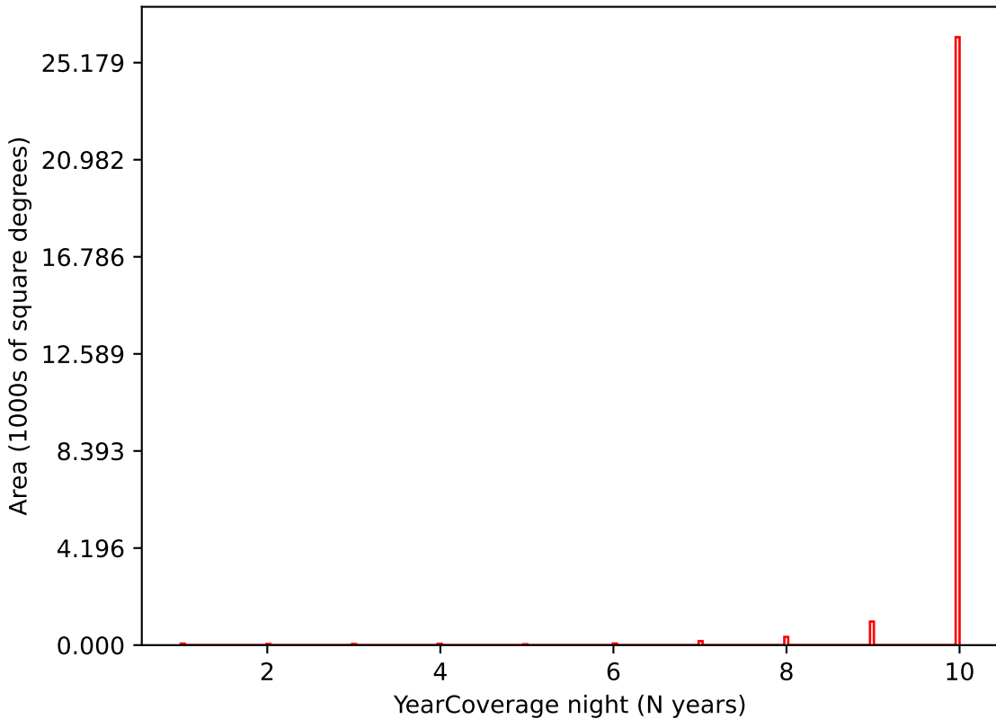
all_long_v3.4_10yrs i band: YearCoverage night
