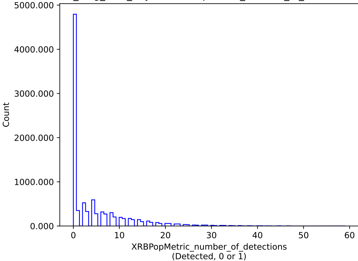
all_long_v3.4_10yrs : XRBPoMetric_number_of_detections
