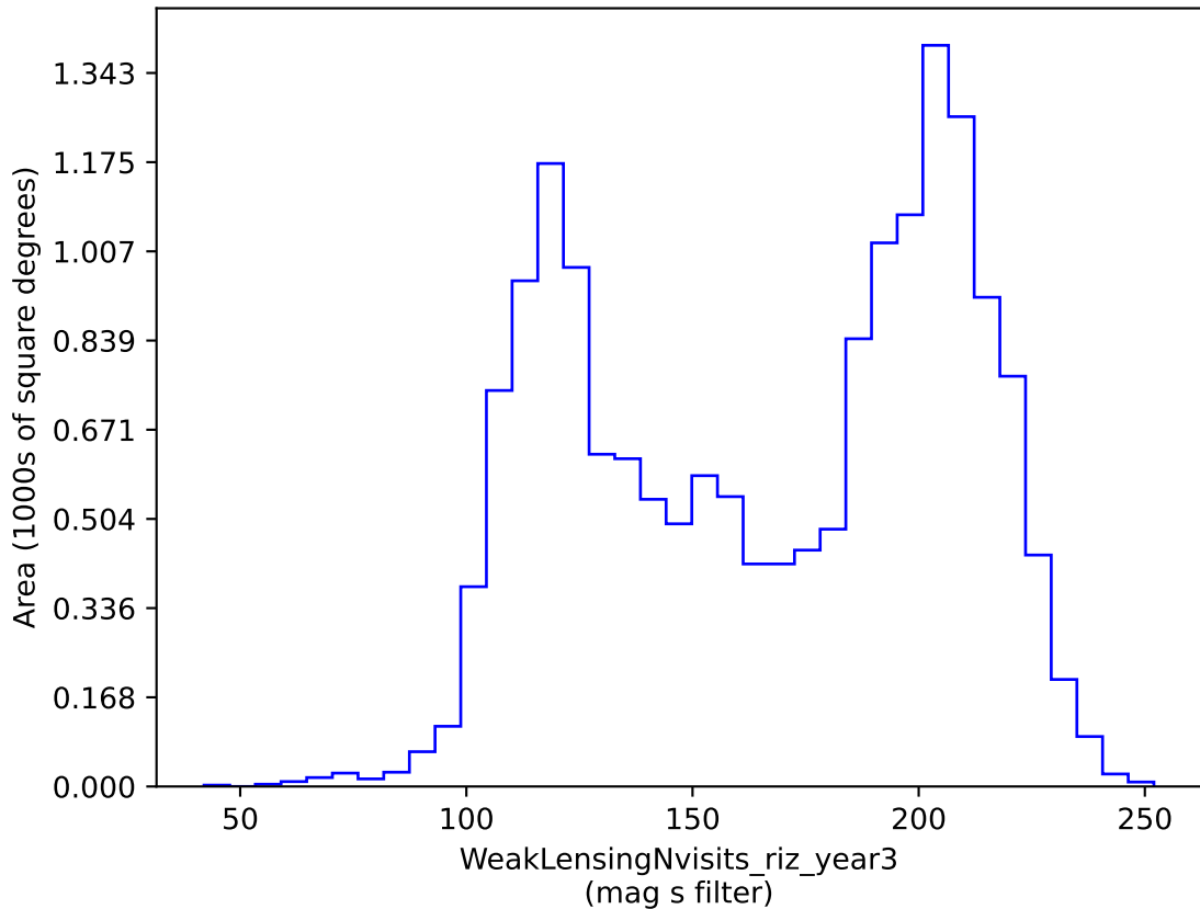
all_long_v3.4_10yrs gri band non-DD: WeakLensingNvisits_riz_year3
