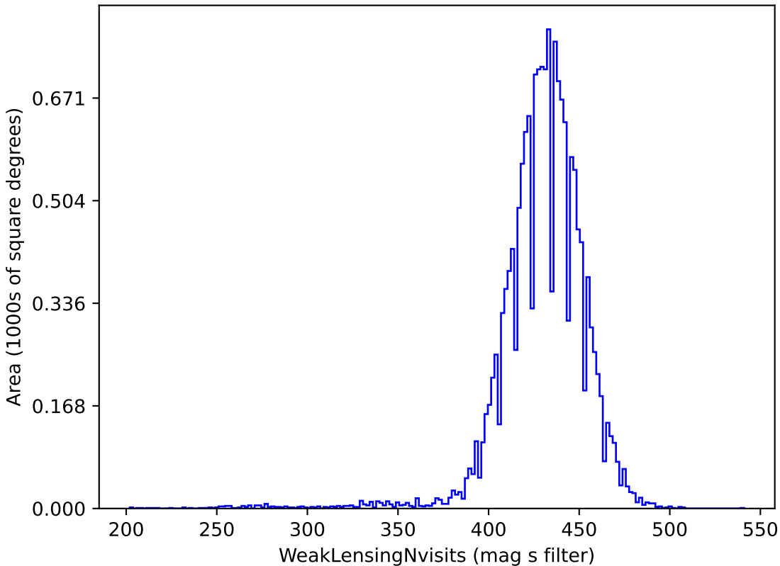
all_long_v3.4_10yrs gri band non-DD: WeakLensingNvisits
