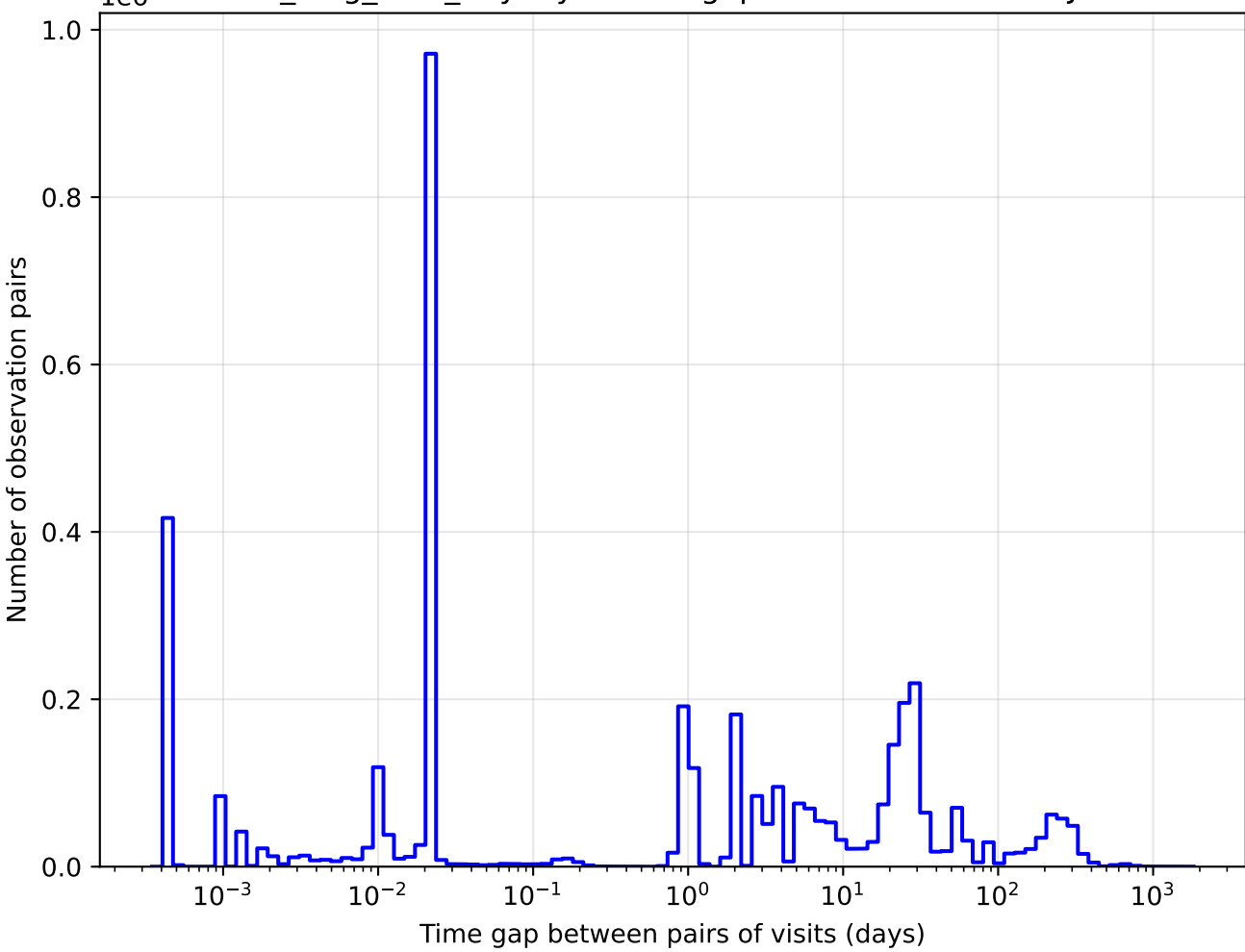
all_long_v3.4_10yrs y band: Tgaps observationStartMJD
